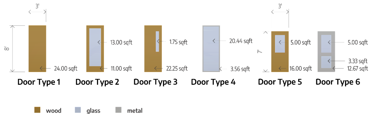
Figure 3. Door types.
